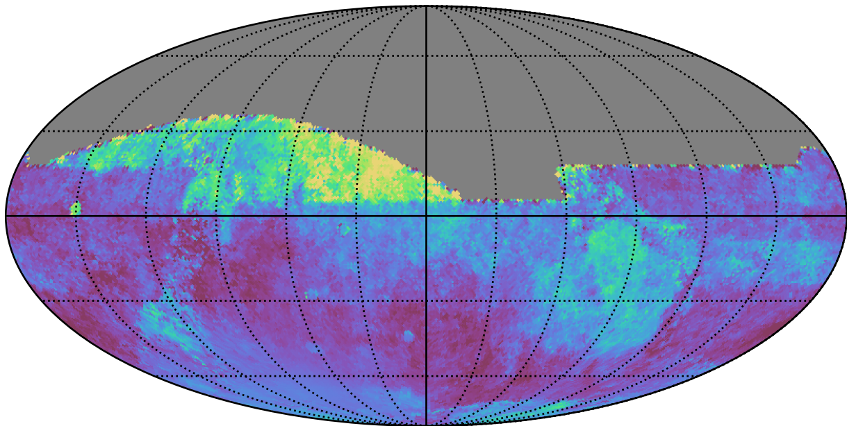
telescope_jerk_v3.5_10yrs All sky all bands: Median moonDistance
