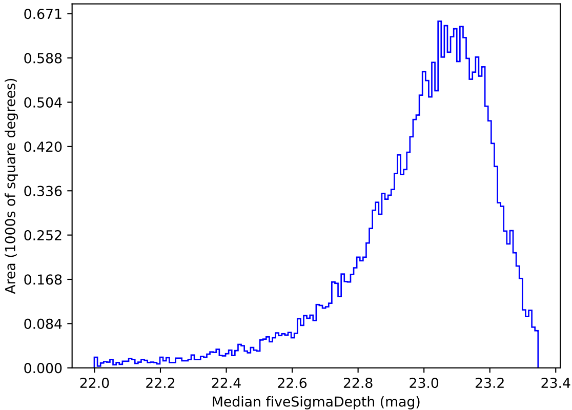
telescope_jerk_v3.5_10yrs Yr 1 z band: Median fiveSigmaDepth
