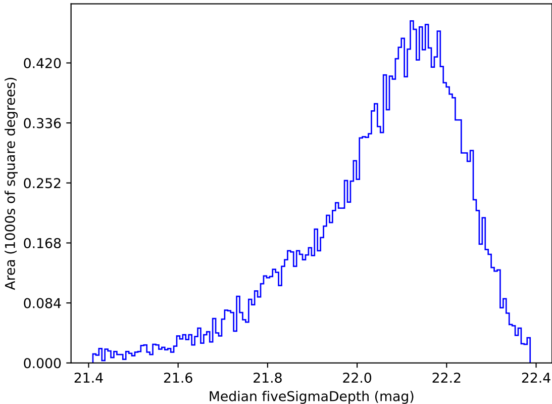
telescope_jerk_v3.5_10yrs Yr 1 y band: Median fiveSigmaDepth
