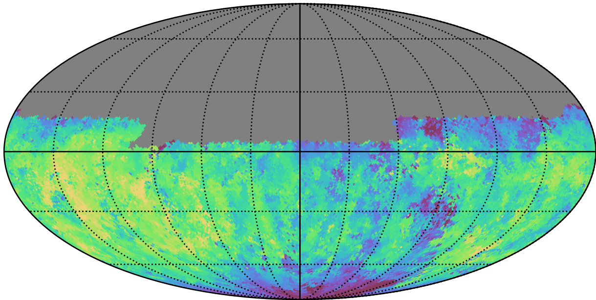
telescope_jerk_v3.5_10yrs Yr 1 u band: Median fiveSigmaDepth
