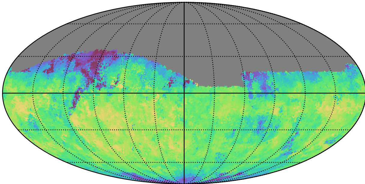
telescope_jerk_v3.5_10yrs Yr 1 i band: Median fiveSigmaDepth
