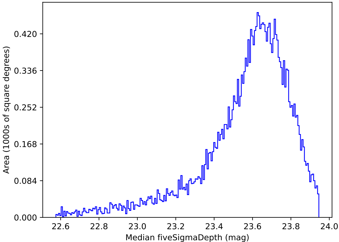
telescope_jerk_v3.5_10yrs Yr 1 i band: Median fiveSigmaDepth
