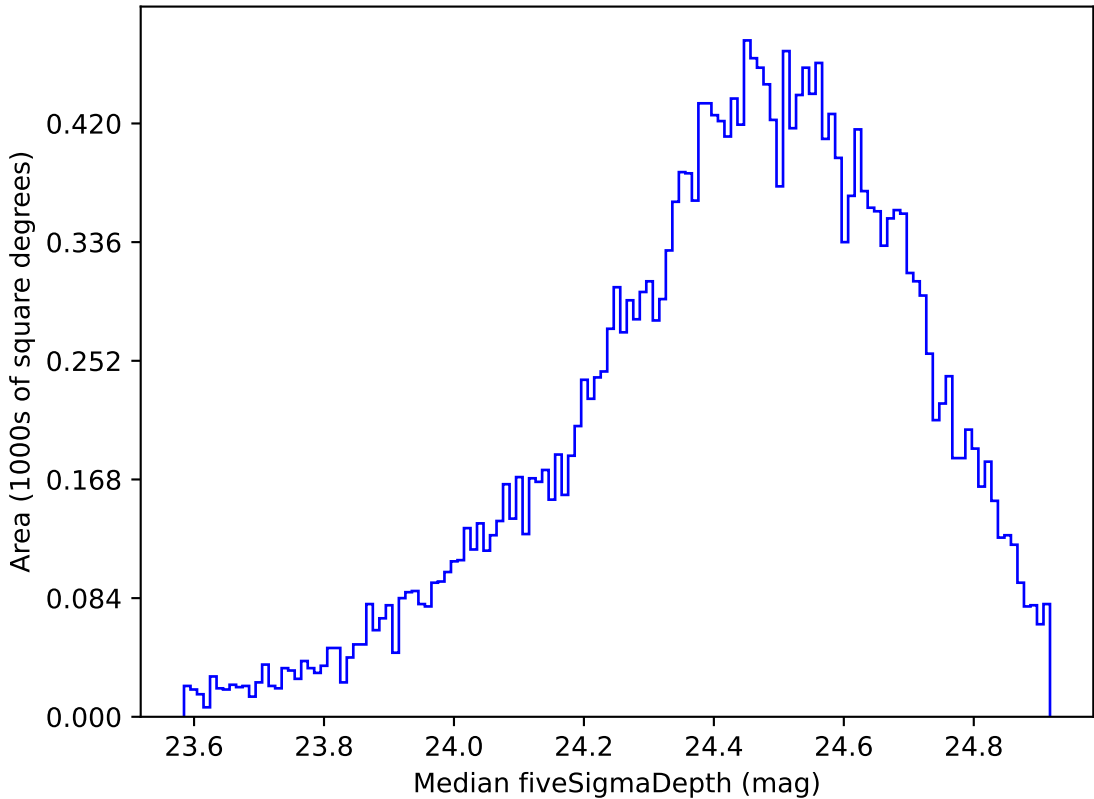
telescope_jerk_v3.5_10yrs Yr 1 g band: Median fiveSigmaDepth
