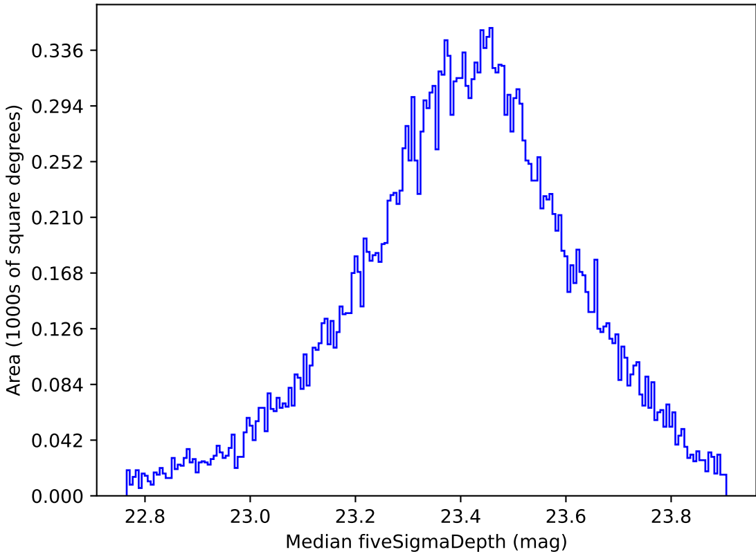
telescope_jerk_v3.5_10yrs Yr 1 all bands: Median fiveSigmaDepth
