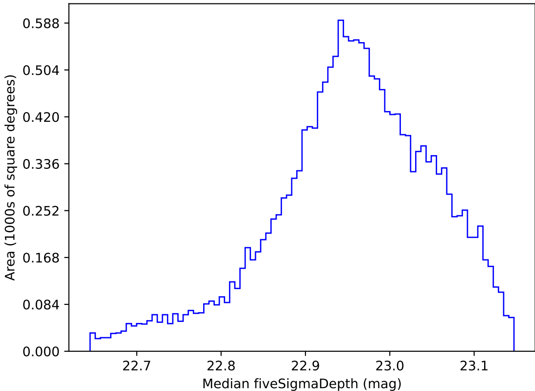
telescope_jerk_v3.5_10yrs WFD z band: Median fiveSigmaDepth
