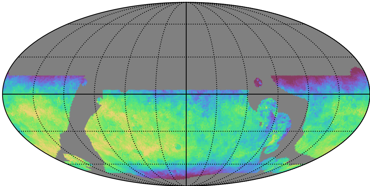
telescope_jerk_v3.5_10yrs WFD y band: Median fiveSigmaDepth
