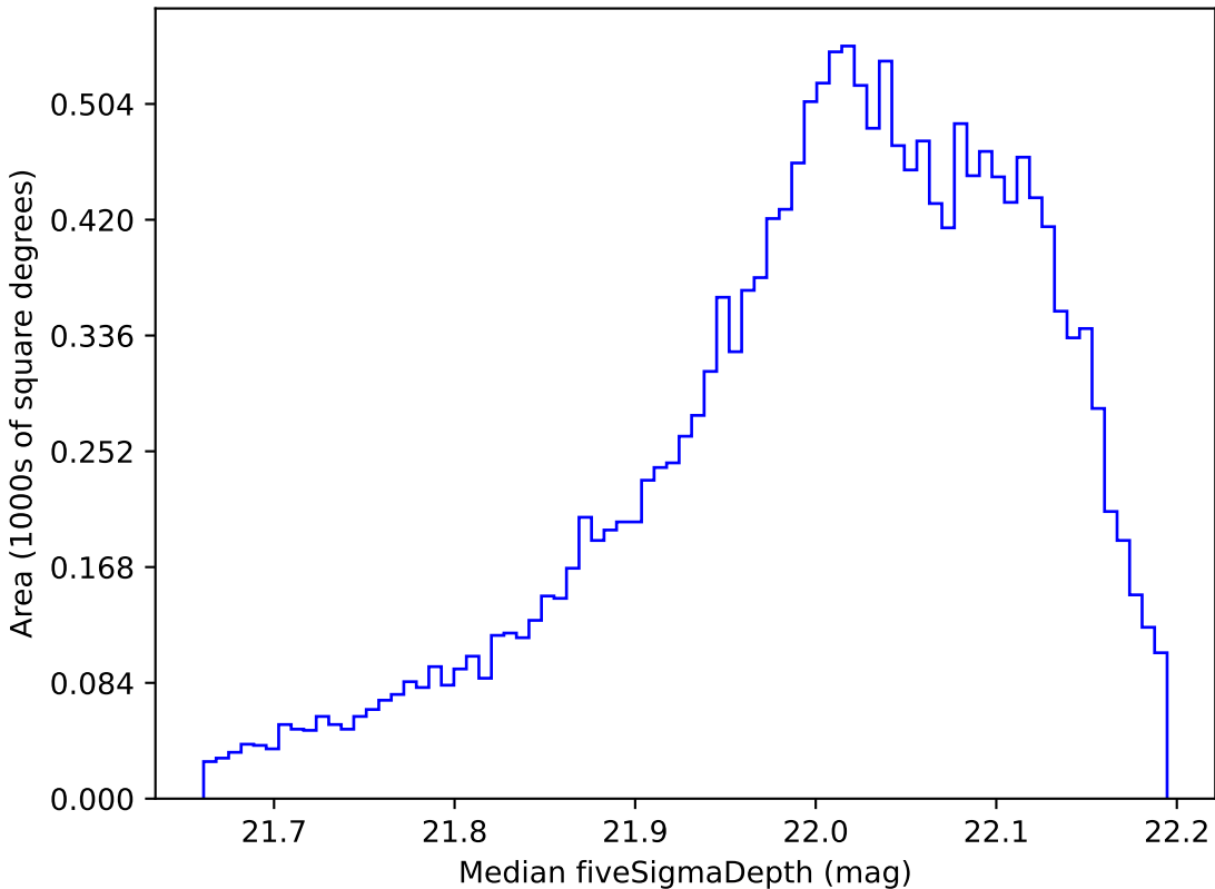
telescope_jerk_v3.5_10yrs WFD y band: Median fiveSigmaDepth
