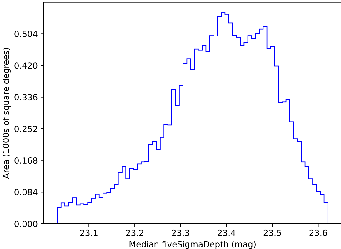
telescope_jerk_v3.5_10yrs WFD u band: Median fiveSigmaDepth
