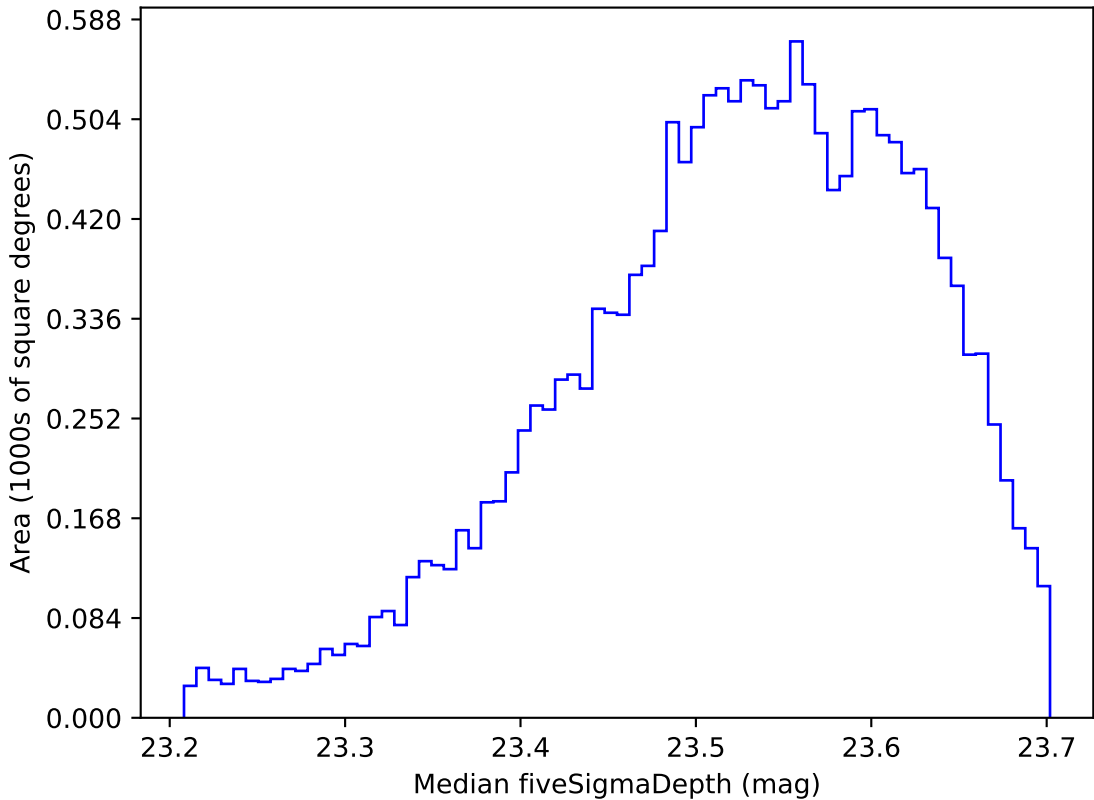
telescope_jerk_v3.5_10yrs WFD i band: Median fiveSigmaDepth
