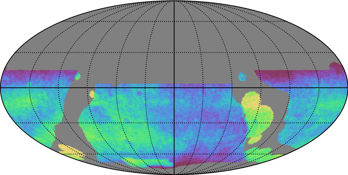
telescope_jerk_v3.5_10yrs WFD all bands: Median fiveSigmaDepth
