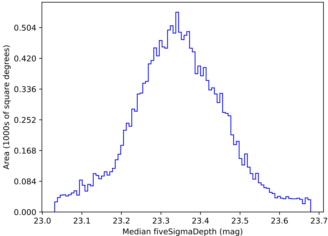
telescope_jerk_v3.5_10yrs WFD all bands: Median fiveSigmaDepth
