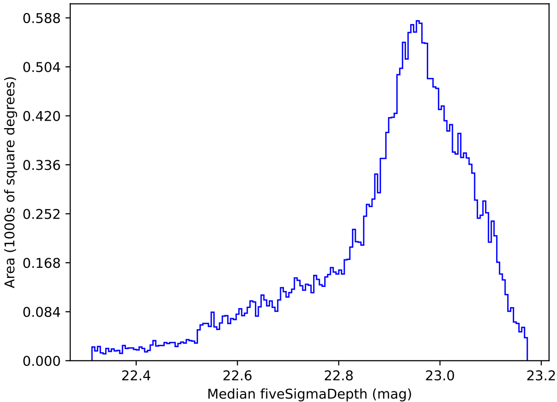
telescope_jerk_v3.5_10yrs All sky z band: Median fiveSigmaDepth
