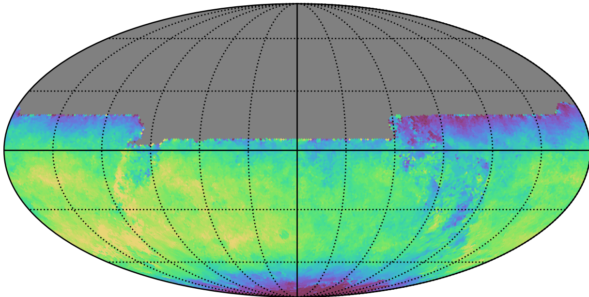
telescope_jerk_v3.5_10yrs All sky y band: Median fiveSigmaDepth
