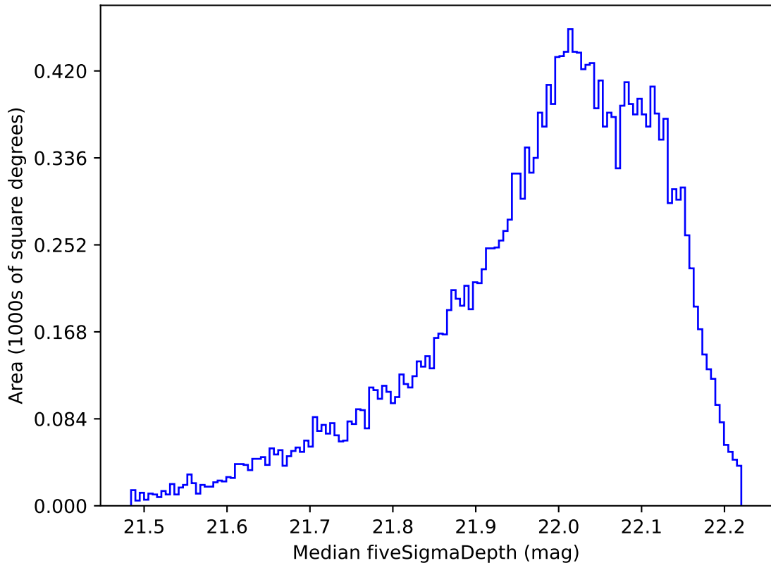
telescope_jerk_v3.5_10yrs All sky y band: Median fiveSigmaDepth
