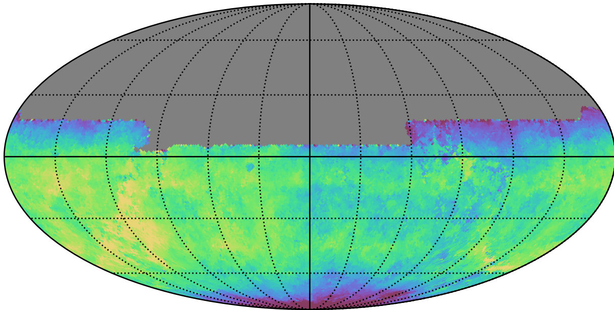
telescope_jerk_v3.5_10yrs All sky u band: Median fiveSigmaDepth
