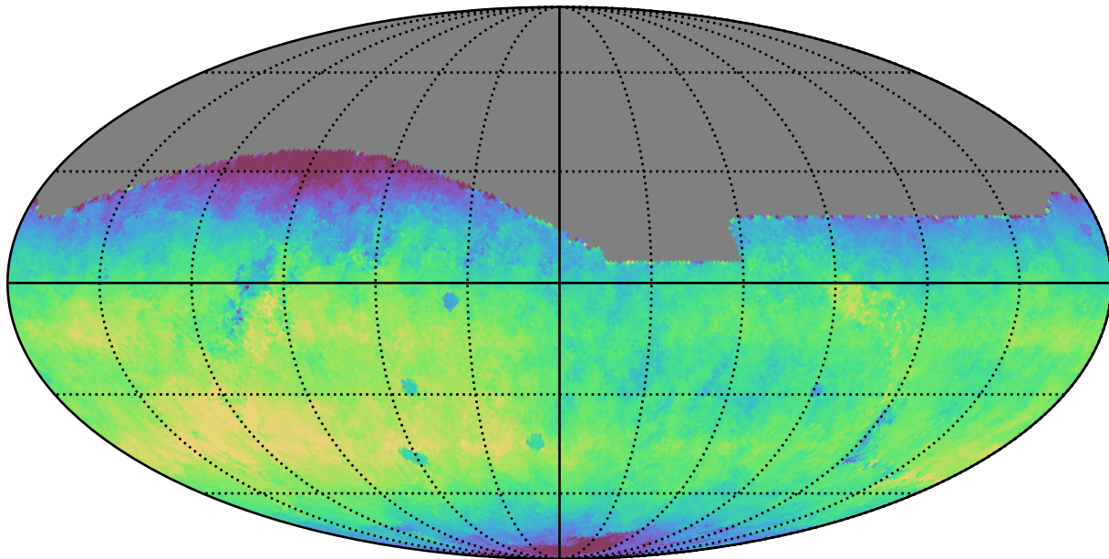
telescope_jerk_v3.5_10yrs All sky r band: Median fiveSigmaDepth
