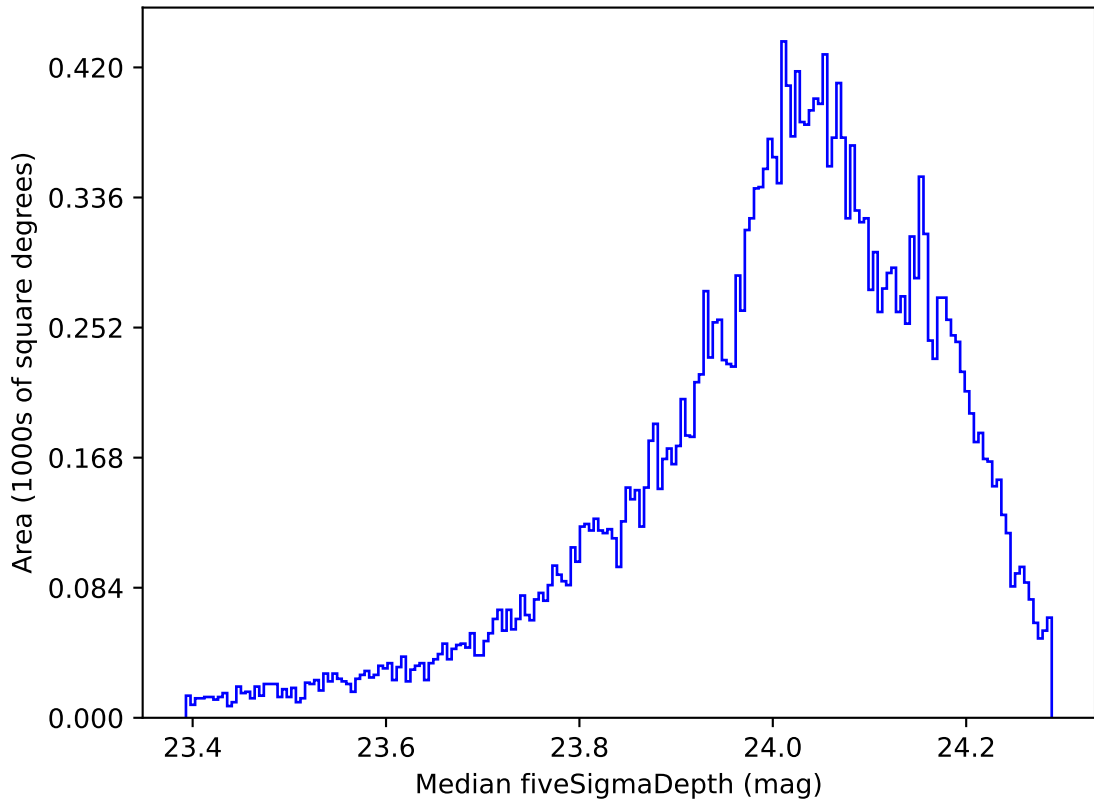
telescope_jerk_v3.5_10yrs All sky r band: Median fiveSigmaDepth
