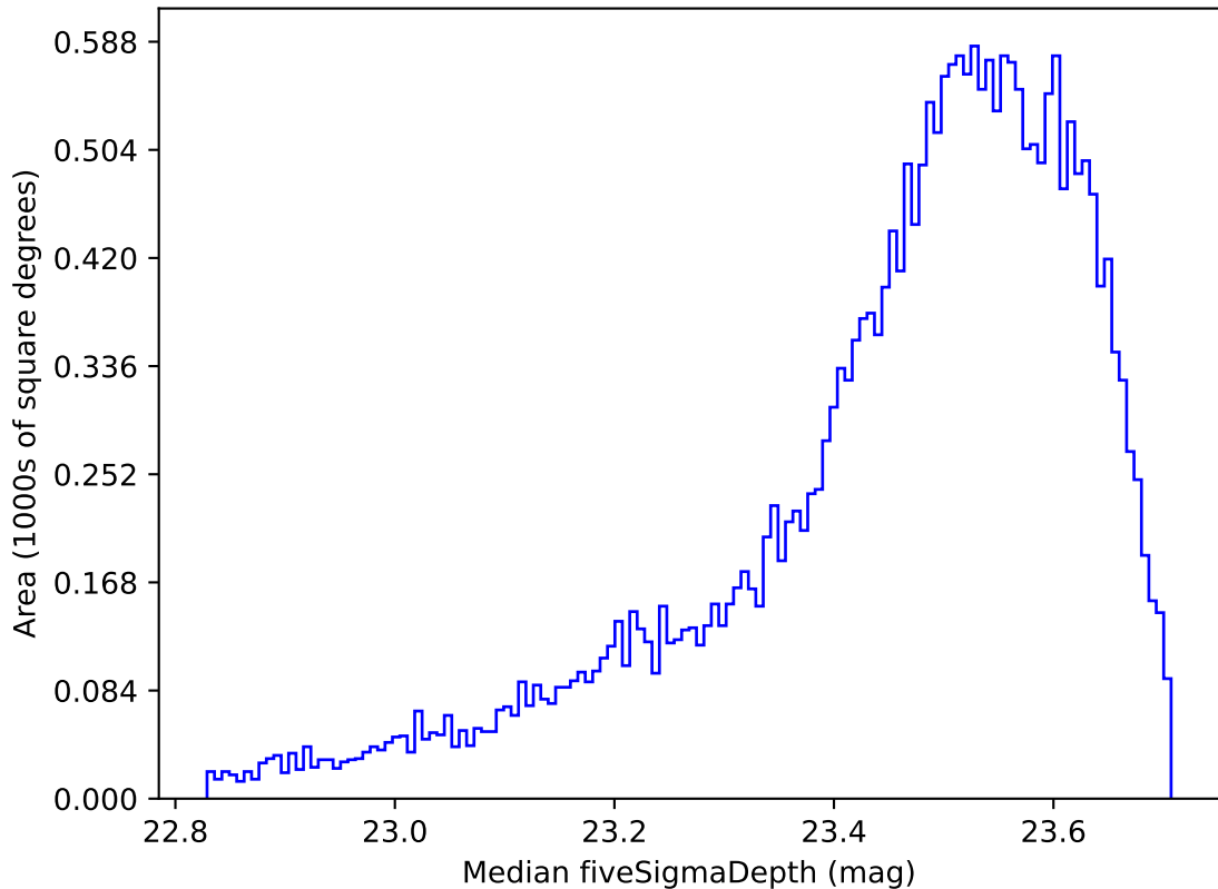
telescope_jerk_v3.5_10yrs All sky i band: Median fiveSigmaDepth
