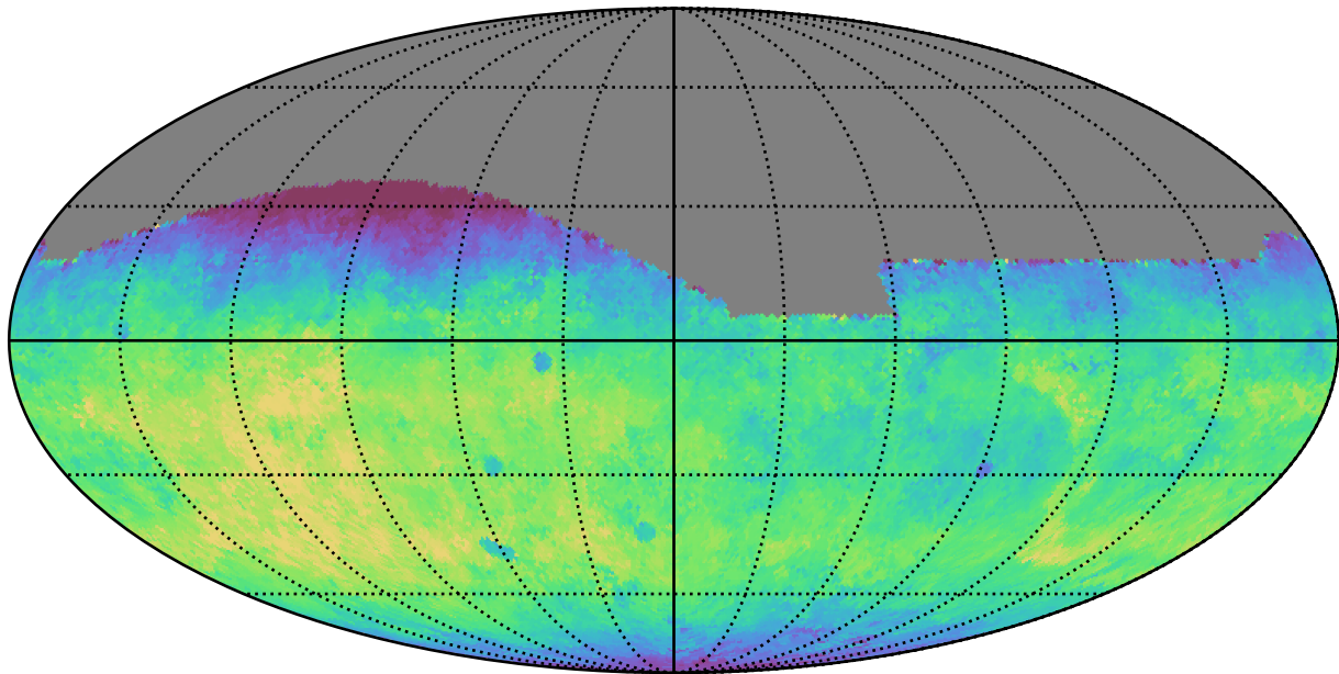
telescope_jerk_v3.5_10yrs All sky g band: Median fiveSigmaDepth
