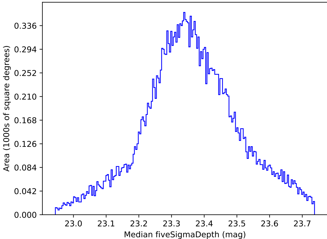
telescope_jerk_v3.5_10yrs All sky all bands: Median fiveSigmaDepth
