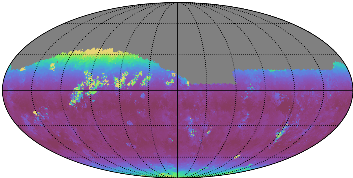
telescope_jerk_v3.5_10yrs Yr 1 z band: Median airmass
