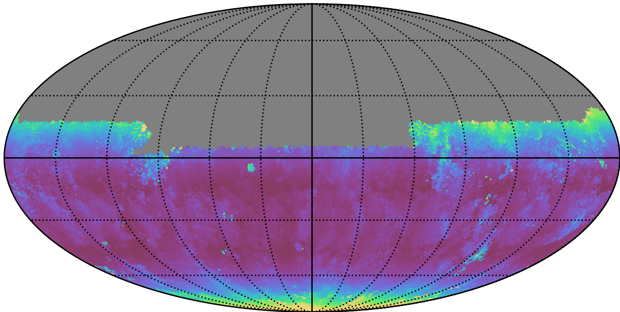
telescope_jerk_v3.5_10yrs Yr 1 y band: Median airmass
