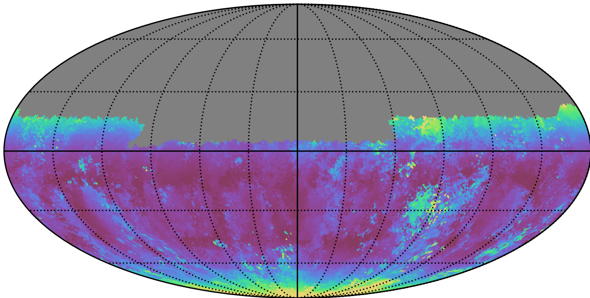
telescope_jerk_v3.5_10yrs Yr 1 u band: Median airmass
