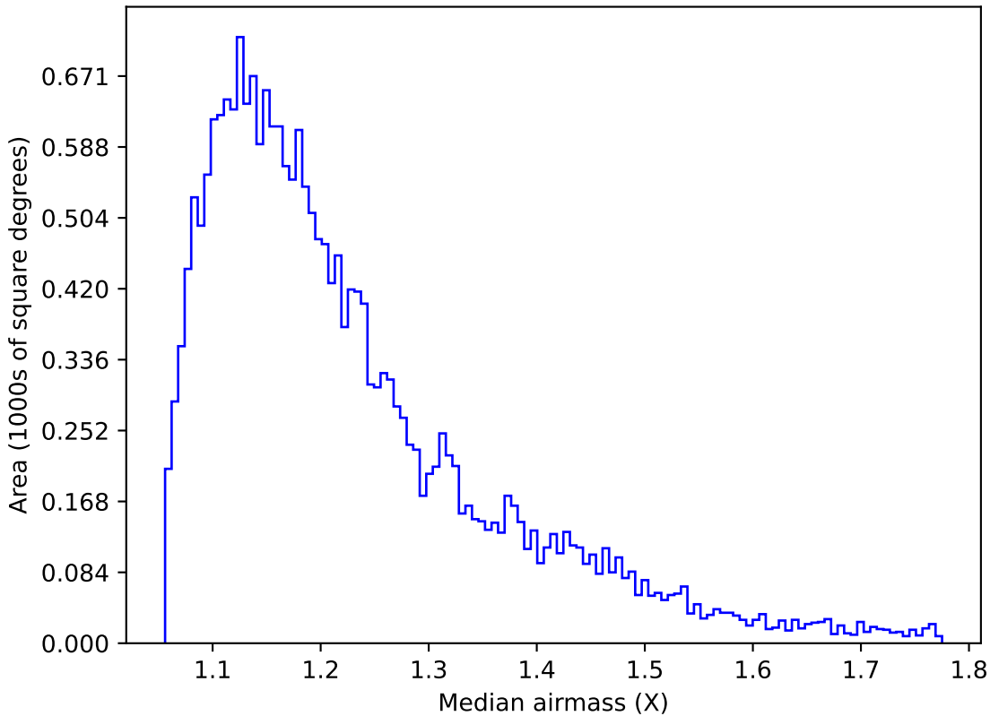
telescope_jerk_v3.5_10yrs Yr 1 u band: Median airmass
