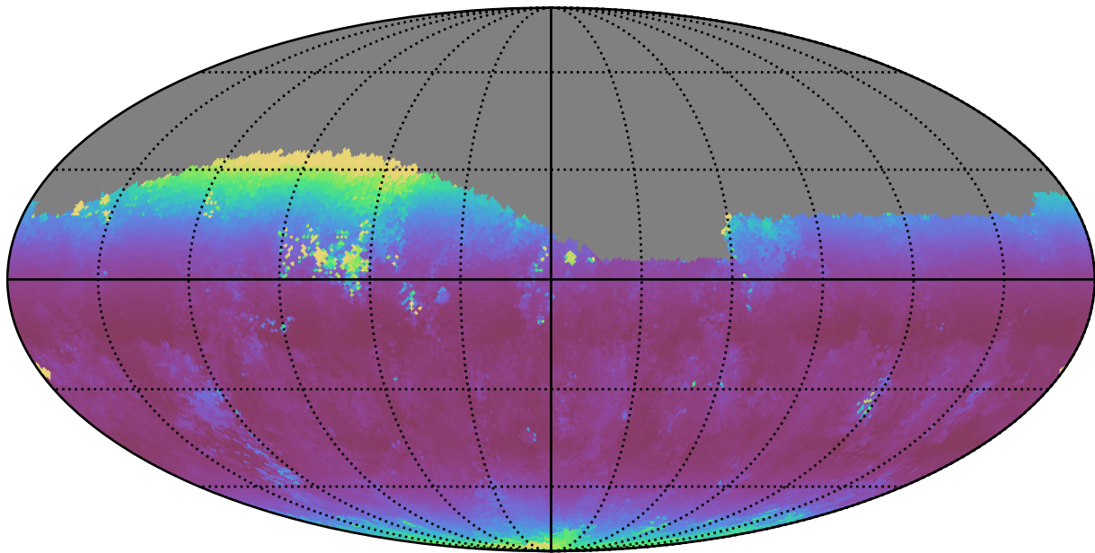
telescope_jerk_v3.5_10yrs Yr 1 r band: Median airmass
