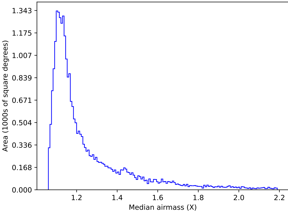
telescope_jerk_v3.5_10yrs Yr 1 r band: Median airmass
