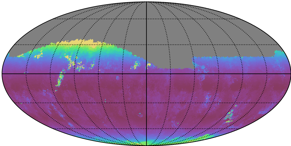
telescope_jerk_v3.5_10yrs Yr 1 i band: Median airmass
