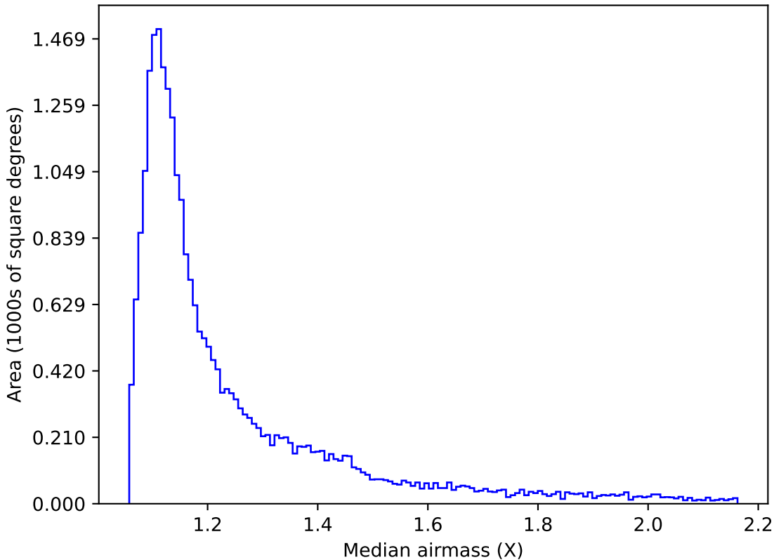
telescope_jerk_v3.5_10yrs Yr 1 i band: Median airmass
