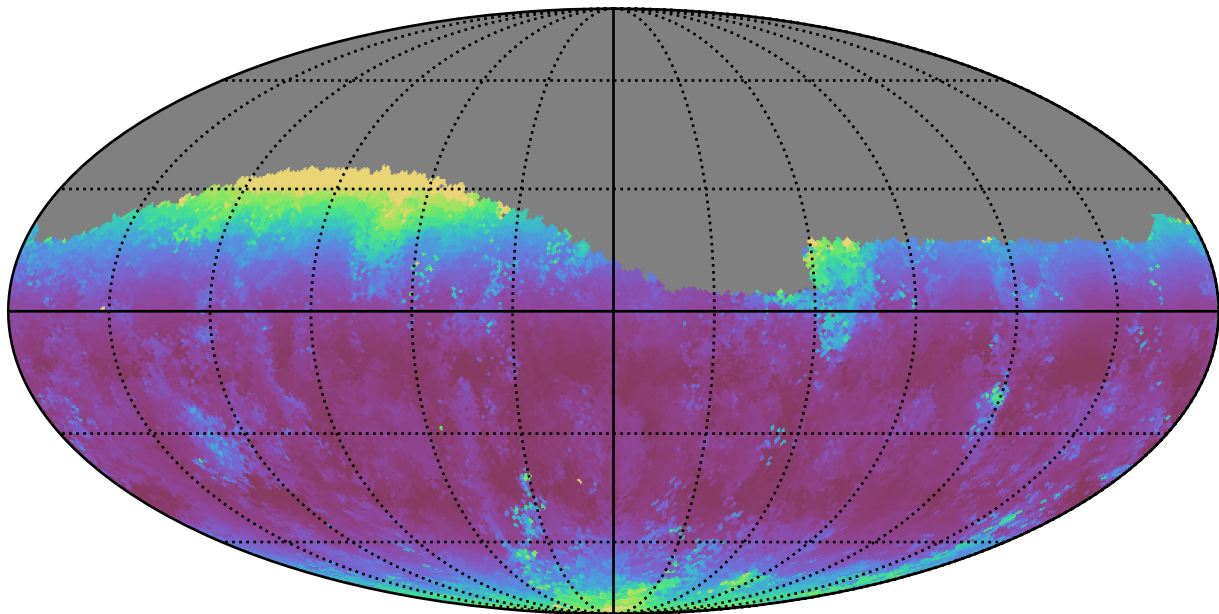
telescope_jerk_v3.5_10yrs Yr 1 g band: Median airmass
