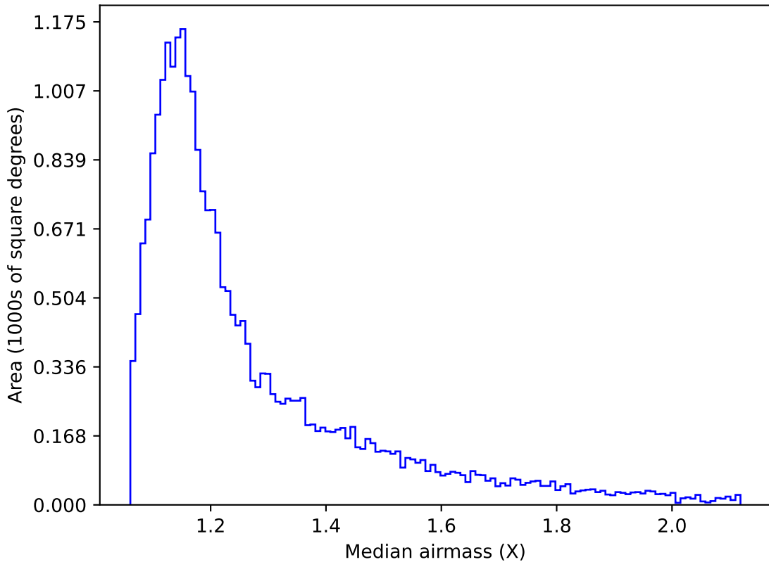
telescope_jerk_v3.5_10yrs Yr 1 g band: Median airmass
