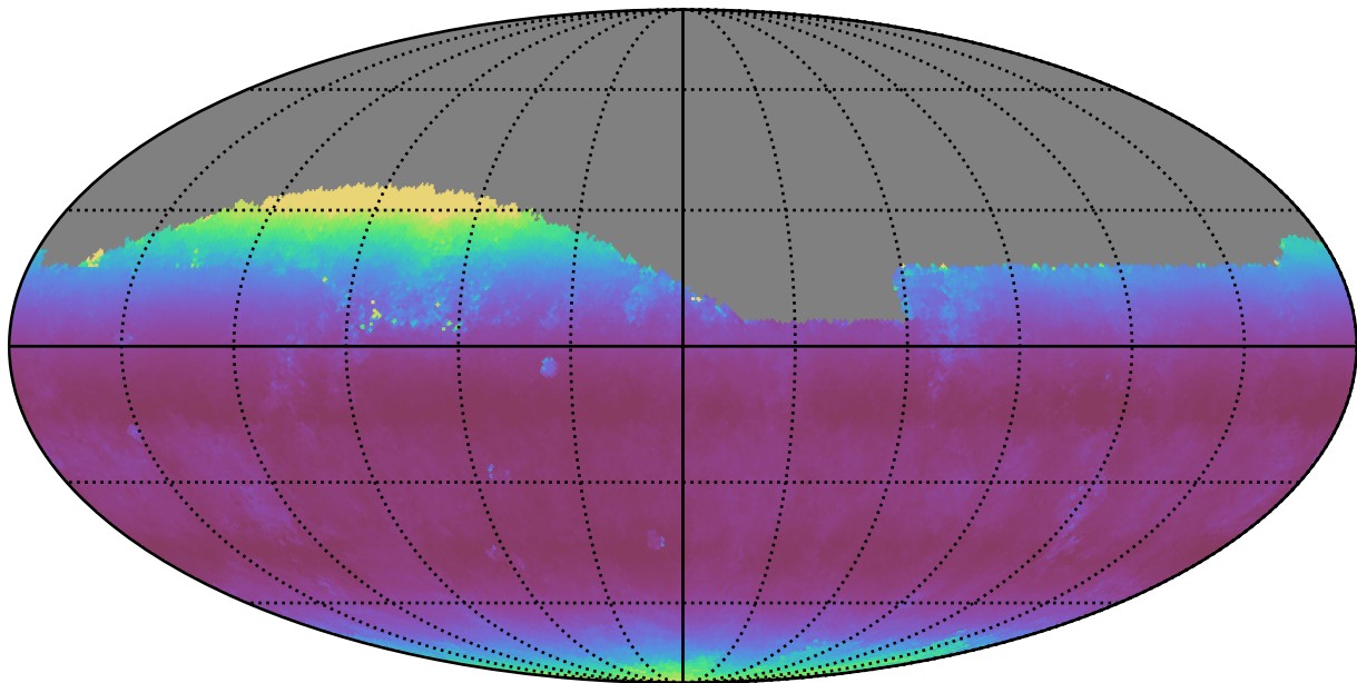
telescope_jerk_v3.5_10yrs Yr 1 all bands: Median airmass
