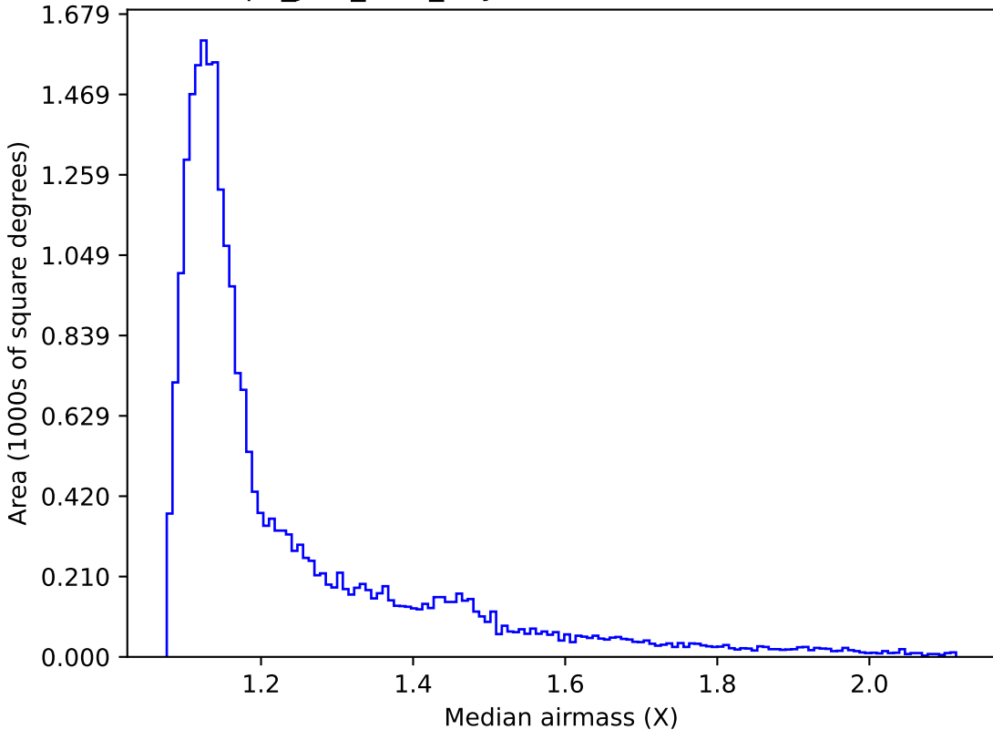
telescope_jerk_v3.5_10yrs Yr 1 all bands: Median airmass
