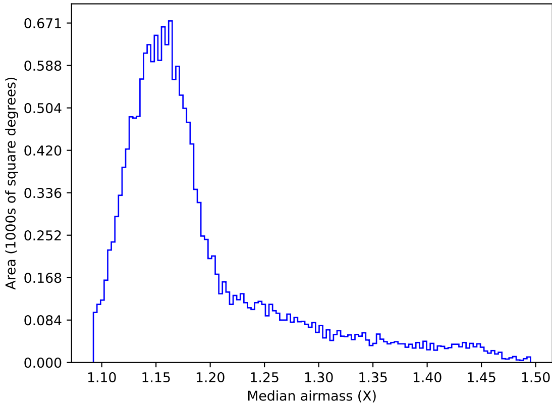
telescope_jerk_v3.5_10yrs WFD z band: Median airmass
