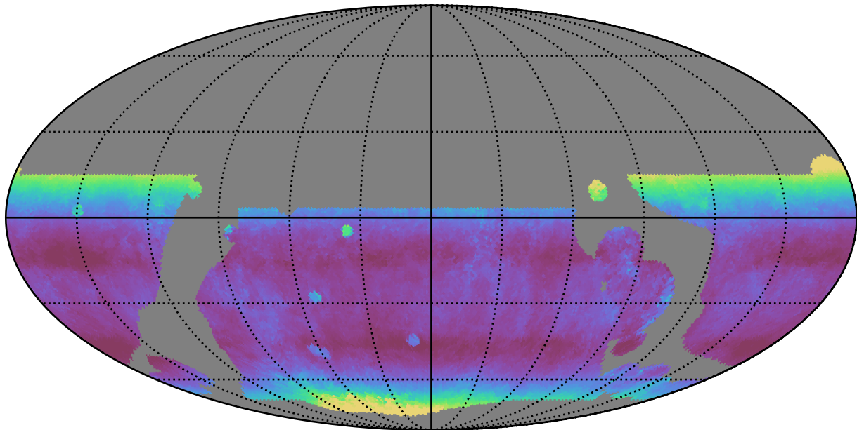
telescope_jerk_v3.5_10yrs WFD y band: Median airmass
