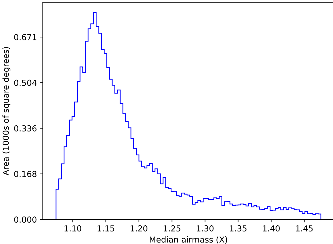
telescope_jerk_v3.5_10yrs WFD u band: Median airmass
