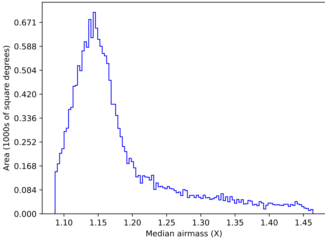
telescope_jerk_v3.5_10yrs WFD i band: Median airmass
