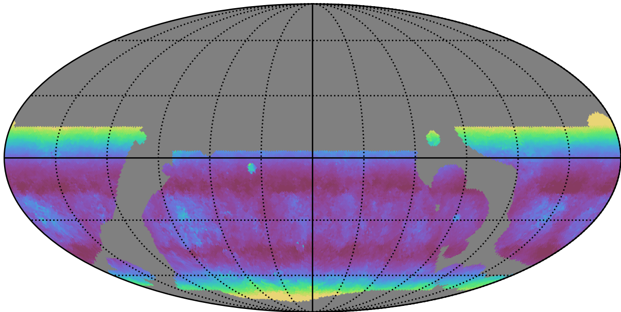
telescope_jerk_v3.5_10yrs WFD g band: Median airmass
