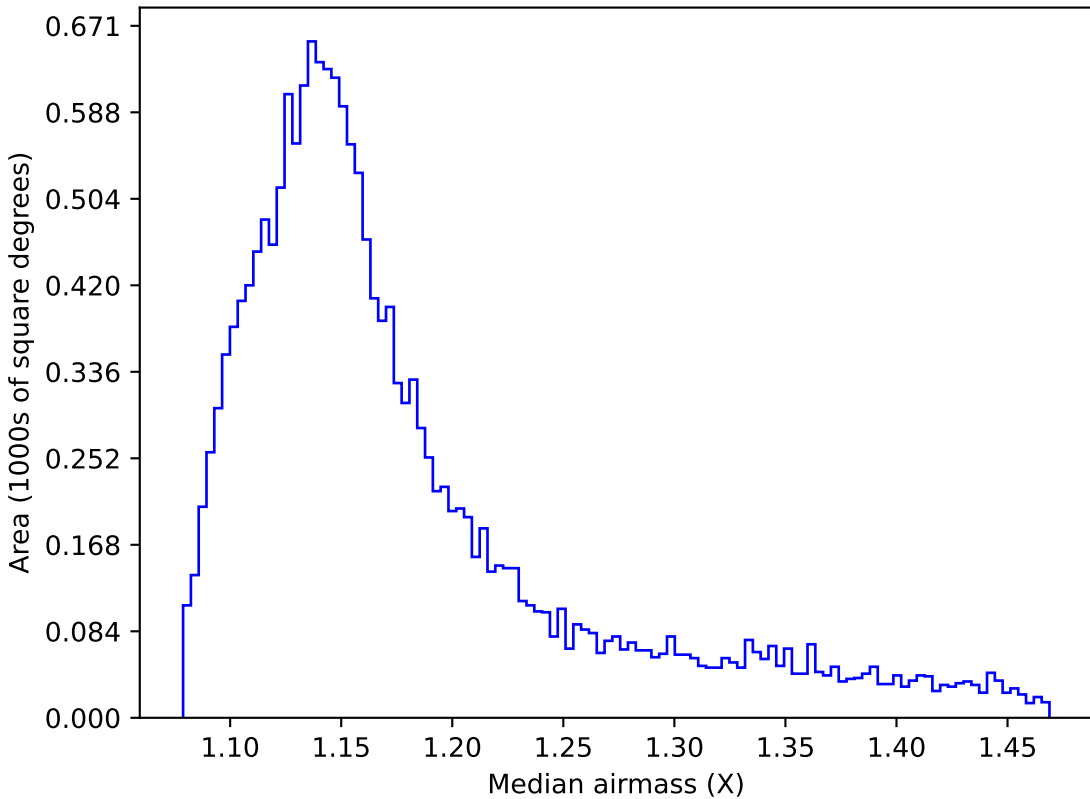
telescope_jerk_v3.5_10yrs WFD g band: Median airmass
