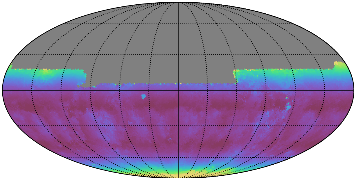
telescope_jerk_v3.5_10yrs All sky u band: Median airmass
