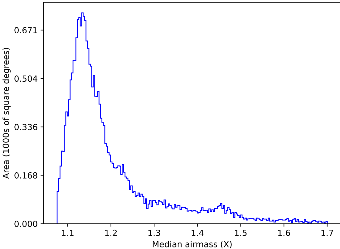
telescope_jerk_v3.5_10yrs All sky u band: Median airmass
