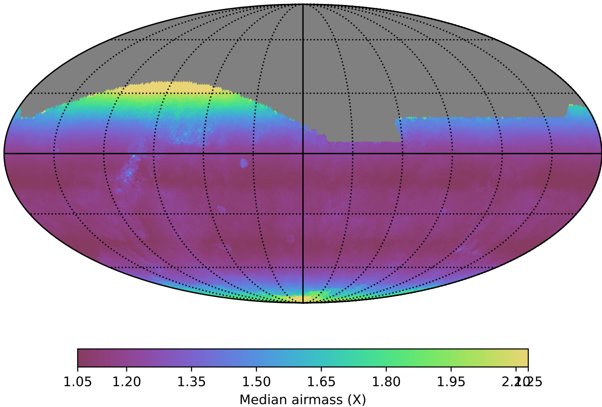
telescope_jerk_v3.5_10yrs All sky r band: Median airmass
