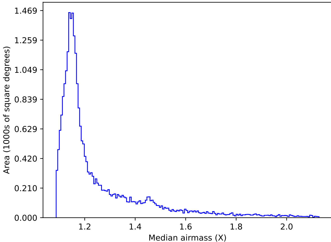
telescope_jerk_v3.5_10yrs All sky r band: Median airmass
