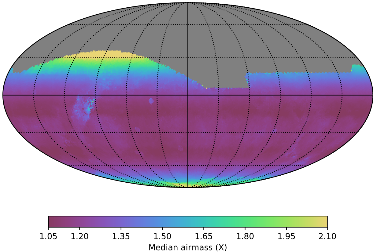
telescope_jerk_v3.5_10yrs All sky i band: Median airmass
