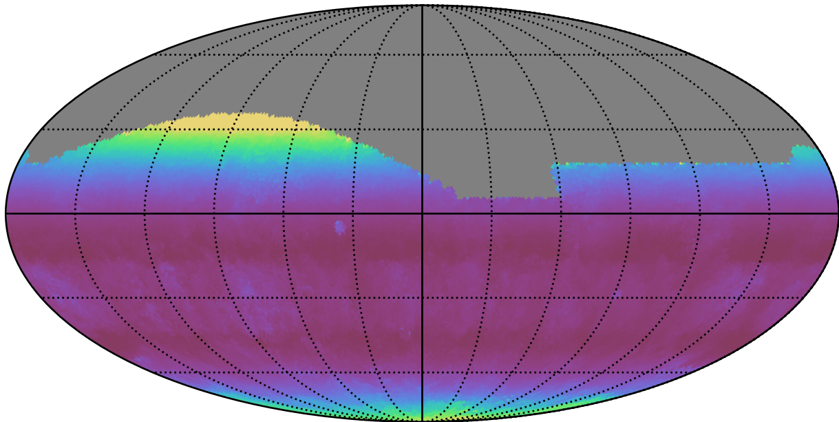
telescope_jerk_v3.5_10yrs All sky g band: Median airmass
