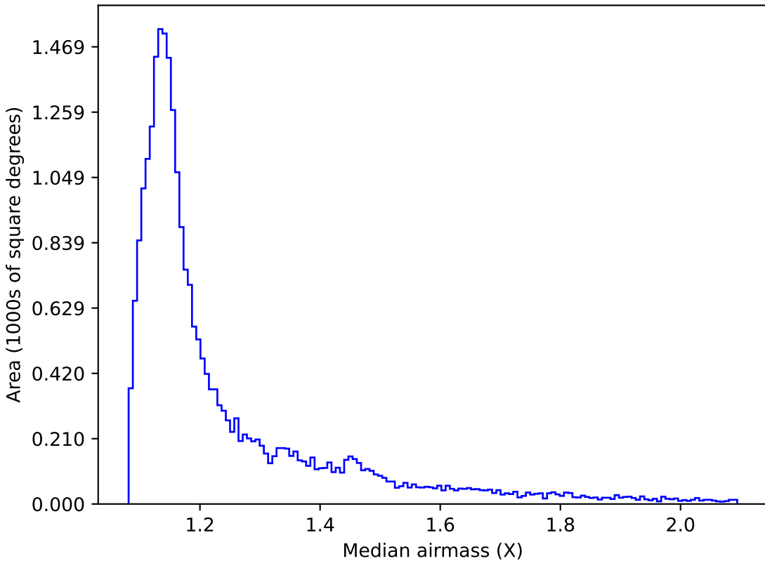
telescope_jerk_v3.5_10yrs All sky g band: Median airmass
