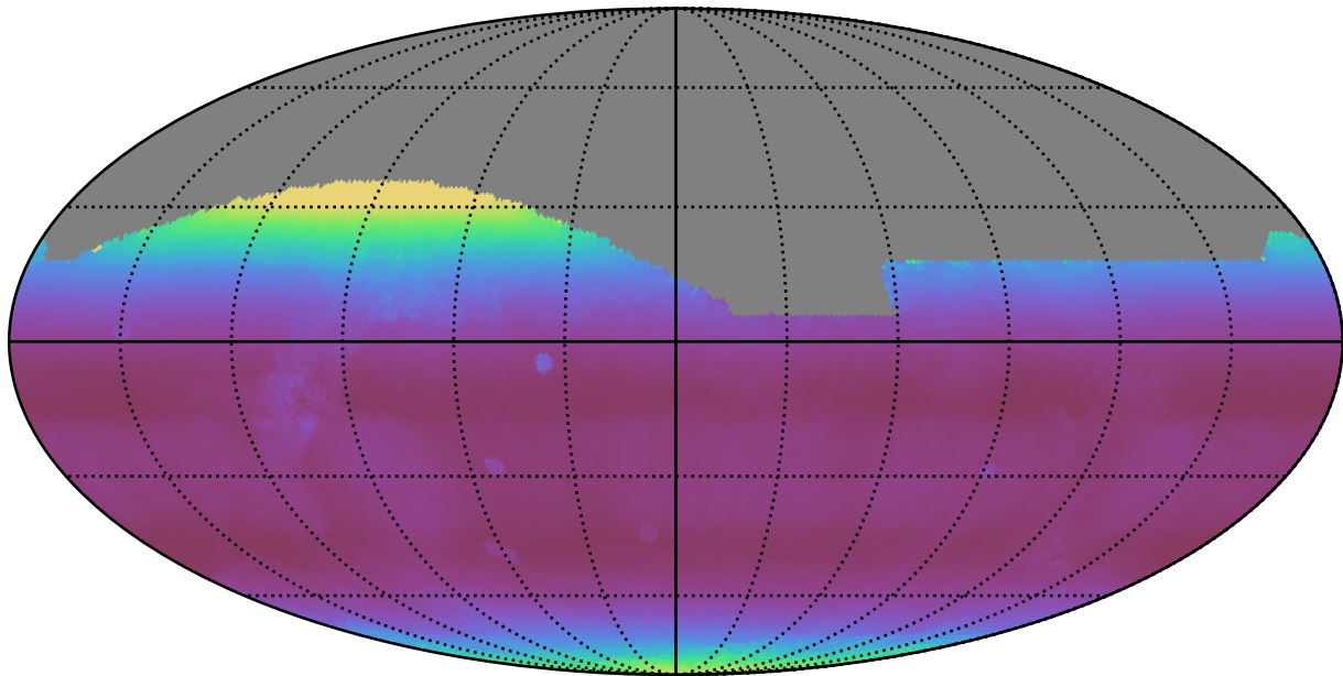
telescope_jerk_v3.5_10yrs All sky all bands: Median airmass
